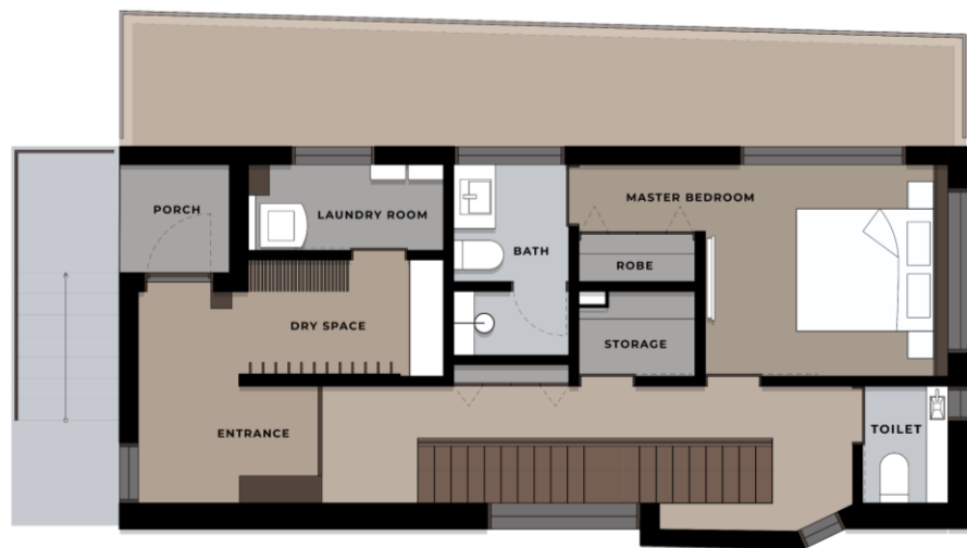
HACHIKO SECOND FLOOR
